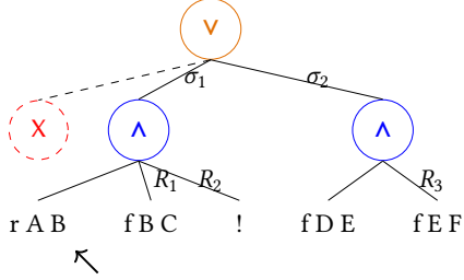
(b) Tree after step on g 0 R
