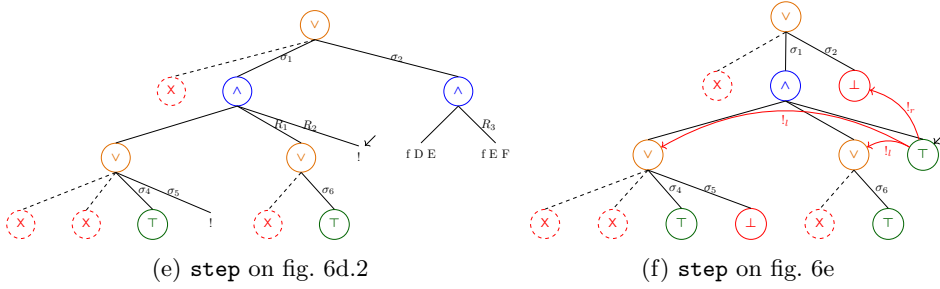
Fig. 6: Execution in the tree semantics. The substitutions \sigma_1 \dots \sigma_6 are from section 2.1. R_1, R_2 , and R_3 are reset points and correspond respectively to the lists of atoms [f \ Y \ Z, !] , [!] , and [f \ Y \ Z] .
