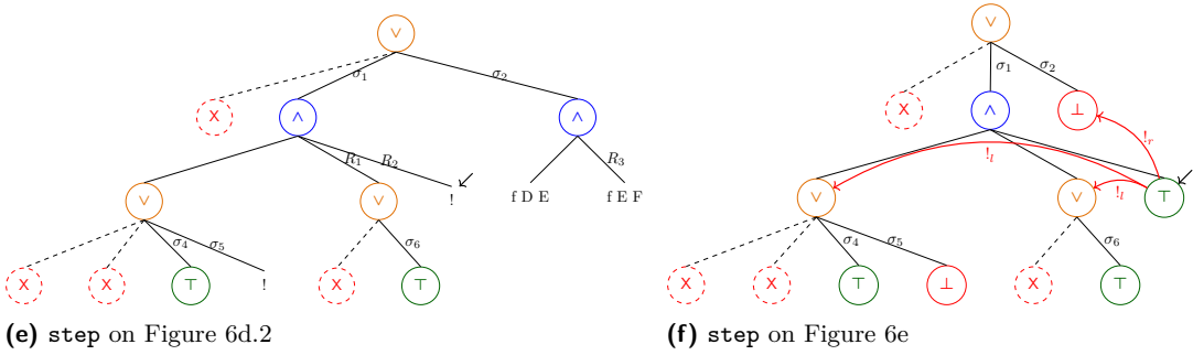
■ Figure 6 Execution in the tree semantics. The substitutions \sigma_1 \dots \sigma_6 are from Section 2.1. R_1, R_2 , and R_3 are reset points and correspond respectively to the lists of atoms [f \ Y \ Z, !] , [!] , and [f \ Y \ Z] .
