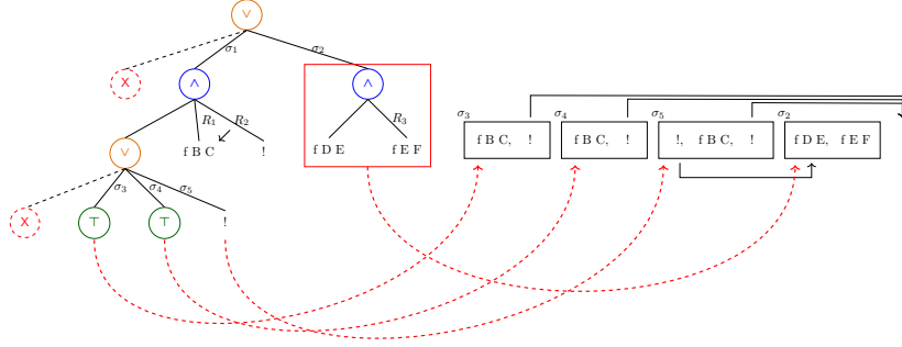
■ Figure 10 Valid tree and Tree to list
