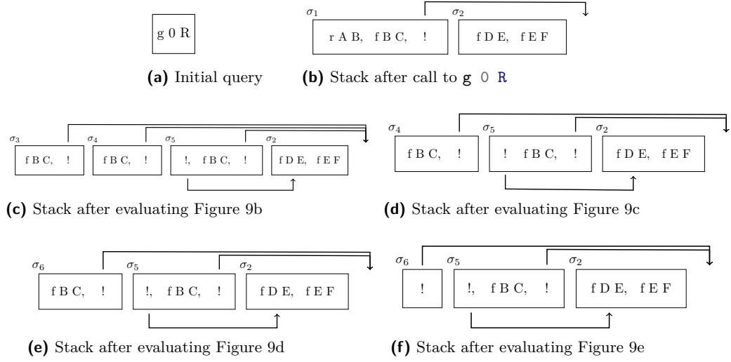
■ Figure 9 Example of execution
