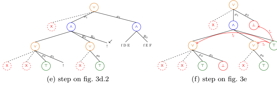
Fig. 3: Execution in the tree semantics. The substitutions \sigma_1 \dots \sigma_6 are from section 2.1. R_1, R_2 , and R_3 are reset points and correspond respectively to the lists of atoms [f \ Y \ Z, !] , [!] , and [f \ Y \ Z] .
