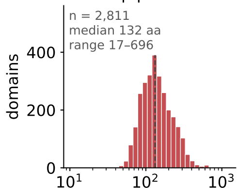
Class d \alpha+\beta proteins
