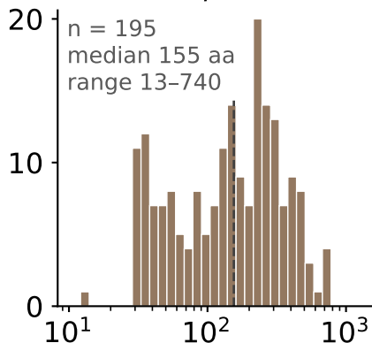
Class f Membrane/cell surface
