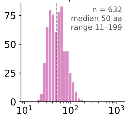
Class g Small proteins
