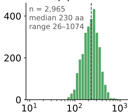
Class g Small proteins
