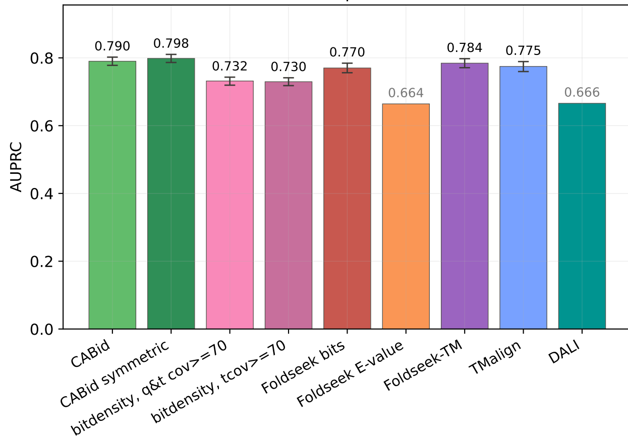
FAMILY | AUPRC
