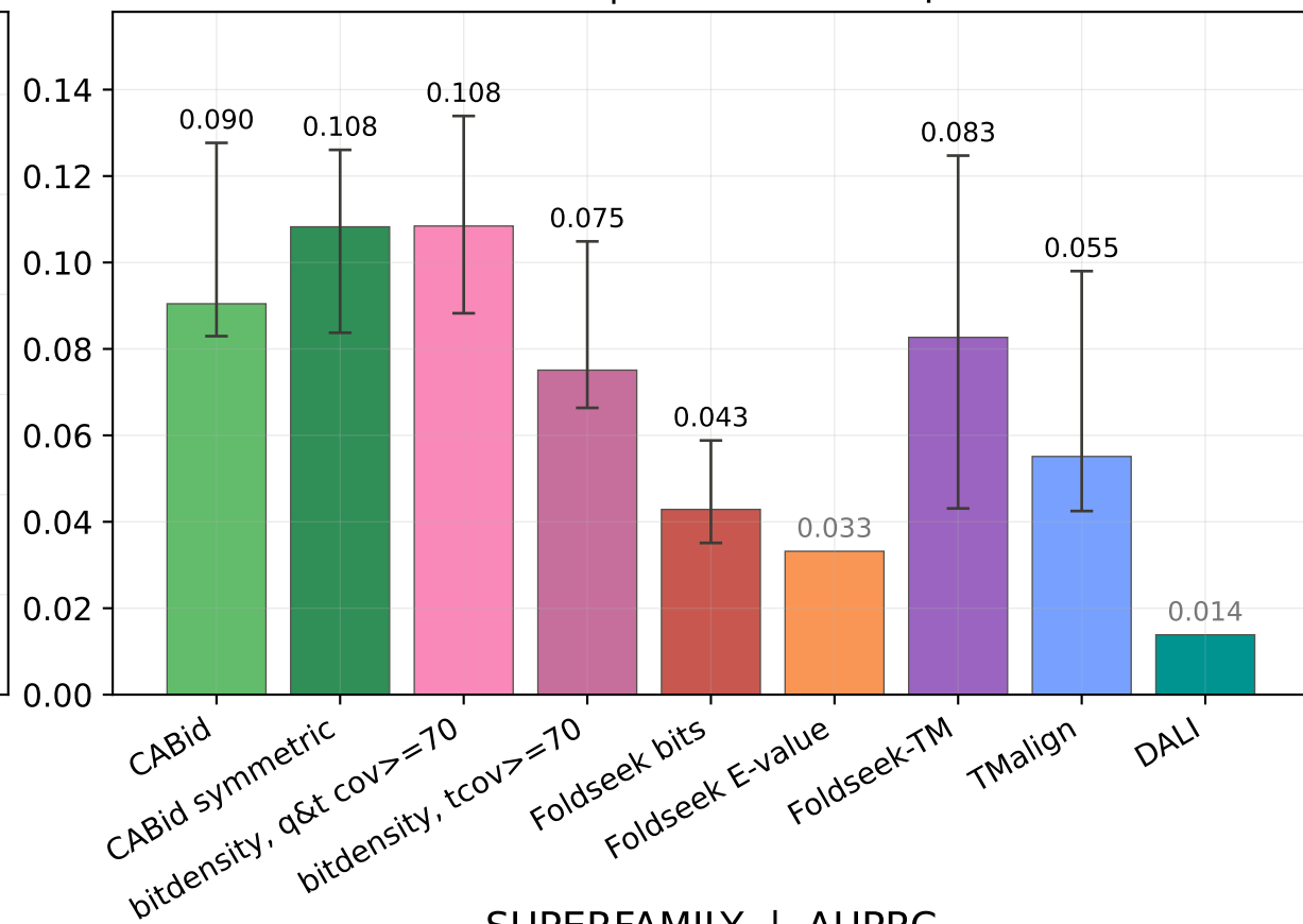
SUPERFAMILY | AUPRC
