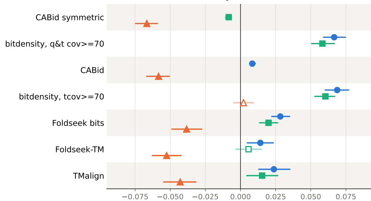
Family · AUPRC
