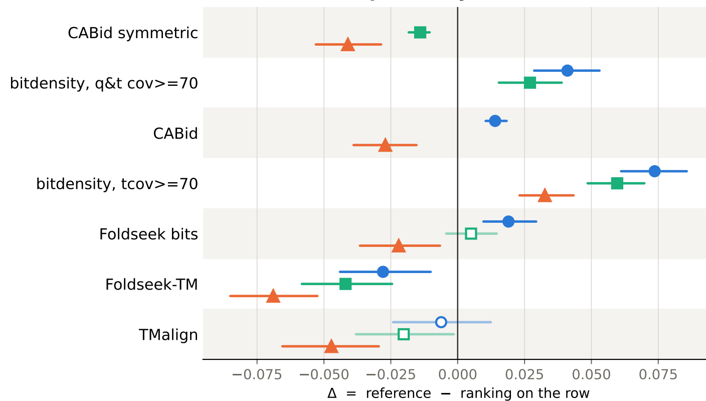
Superfamily · AUPRC
