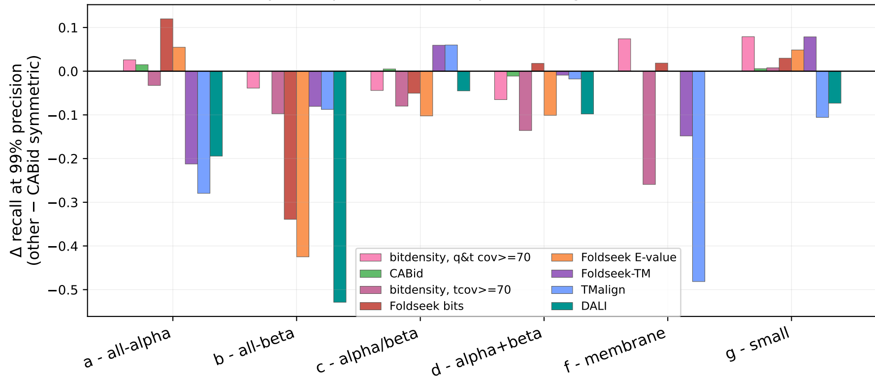
Family level, per class: CABid symmetric against each baseline
