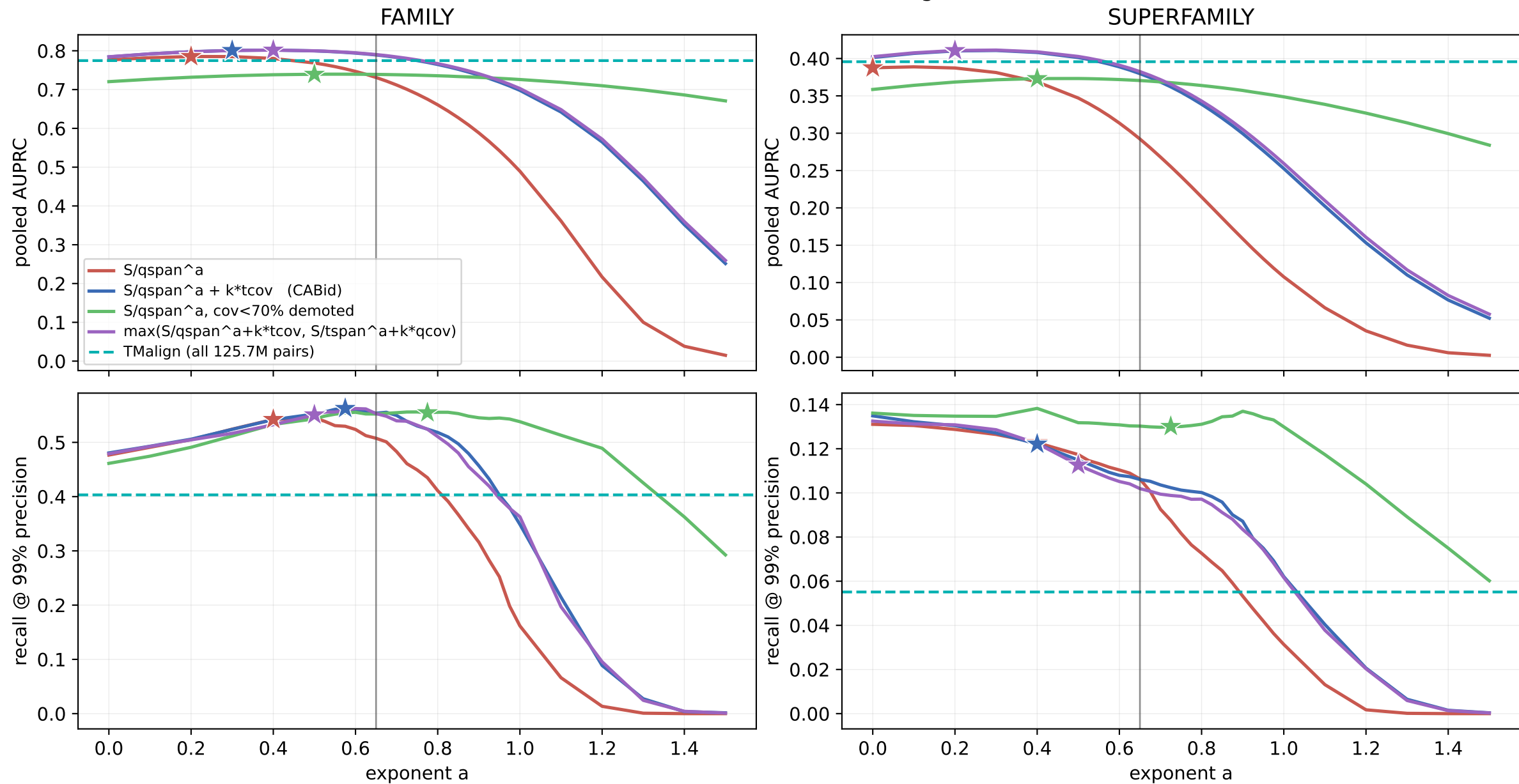
Grouped 5-fold CV over SCOPe folds. Held-out mean across folds. Stars = a* selected on the training folds
