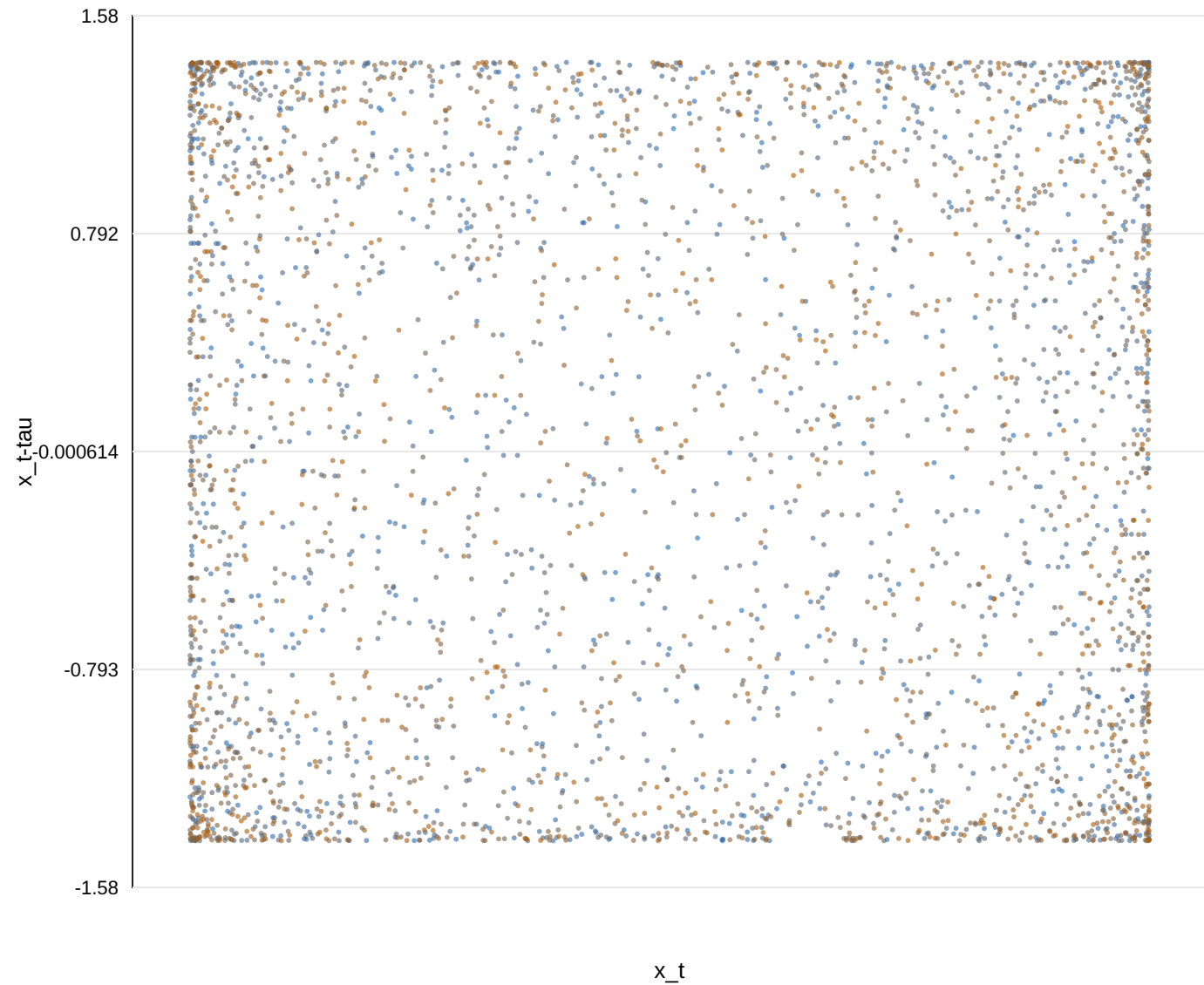
Embedding 2D logistic_clean: tau=9
