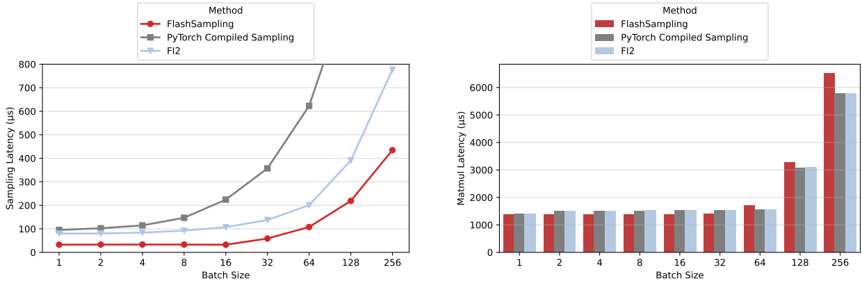
Figure 4 Sampling runtime (left) and matmul runtime (right) in \mu s vs. batch size. Lower is better.
