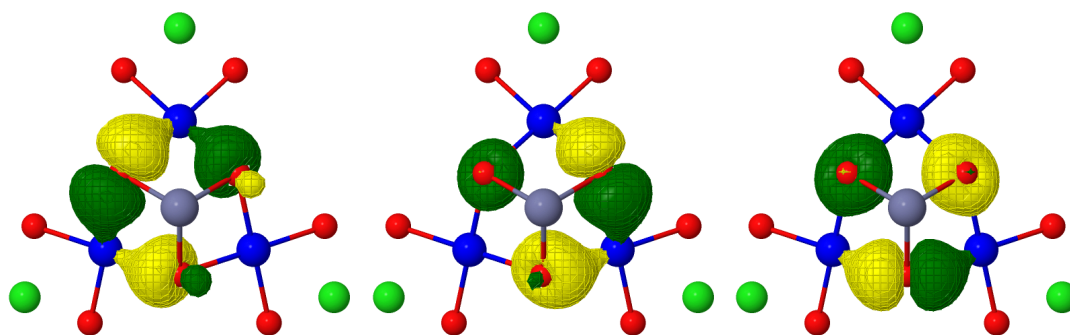
Bridging orbitals from the CAS(9,6) calculation.
