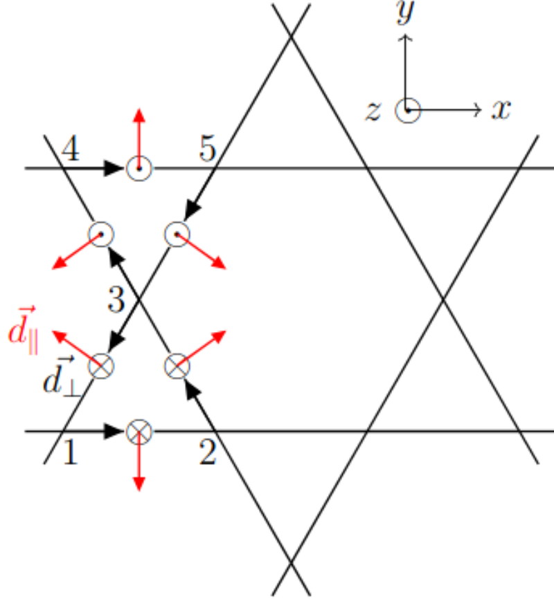
Figure 5.9: Schematic representation of the DMI vector components in two adjacent \text{Cu}^{2+} triangles of the lattice. The black arrows between the magnetic centers indicates the order of the first and second spins in the vector products of the DM interactions. The out-of-plane components alternate from one triangle to its neighbors and point in the opposite direction to the position of the oxygens. The angle between the in-plane components of the vectors within the triangle is 120^\circ .
