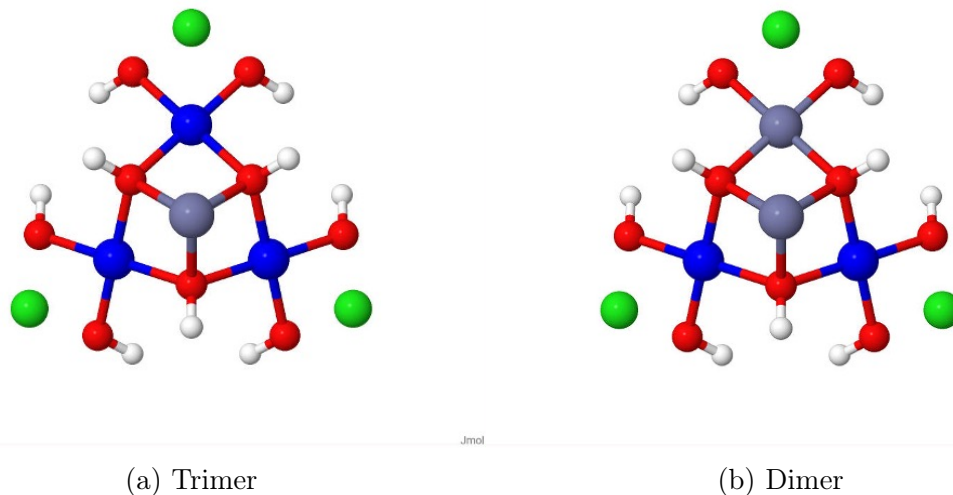
Figure 5.6: Trinuclear and dinuclear embedded clusters used for Wave-function computation
