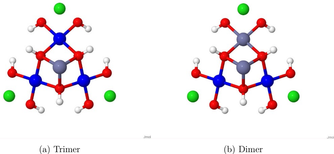
Figure 5.6: Trinuclear and dinuclear embedded clusters used for Wave-function computation
