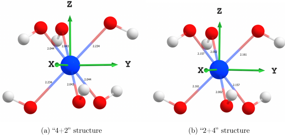
Figure 5.4: Close environment of intersite \text{Cu}^{2+} in both structure obtained via DFT with the B3LYP functional. Bond lengths are in Angstrom
