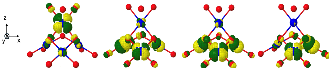
Figure 5.6: CAS(4,4)SCF active orbitals calculated for a tetra-nuclear fragment constituted of three in-plane (below) and an inter-plane (above) copper ions.
