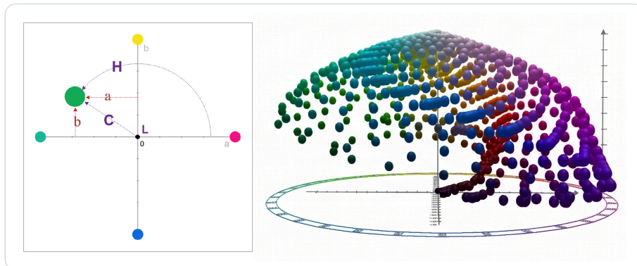
Figure 6: A visual representation of the CIELAB/CIELCH coordinate dimensions, mapping perceptual lightness ( L ), chromatic axes ( a, b ), chroma ( C ), and hue ( H ). [13], [14]
