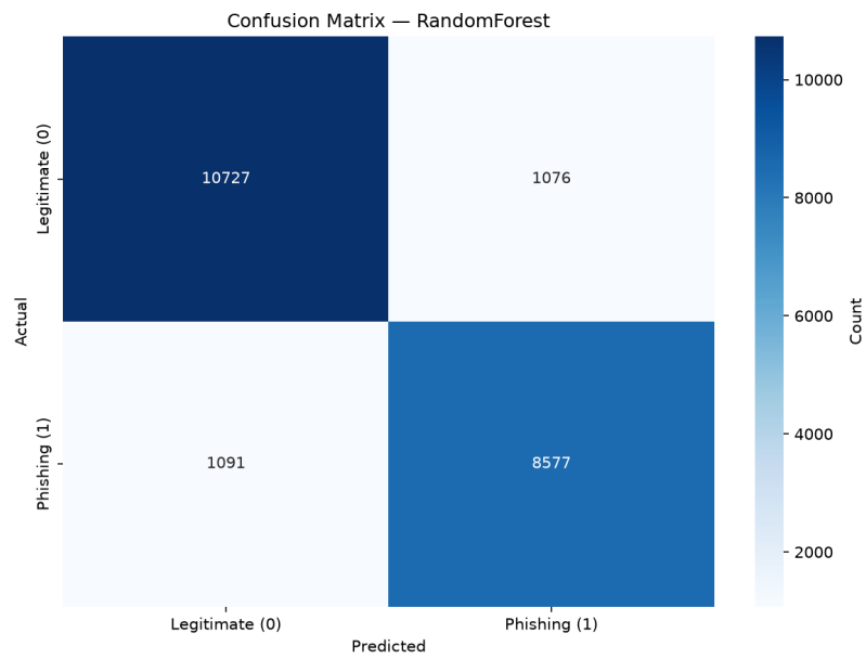
Figure 1. RandomForest confusion matrix (evaluation harness output).
