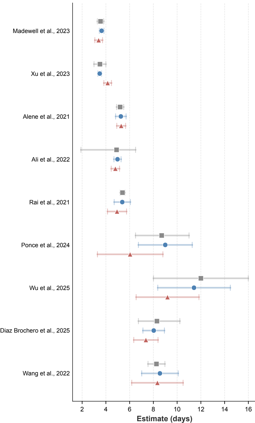
A Serial interval
