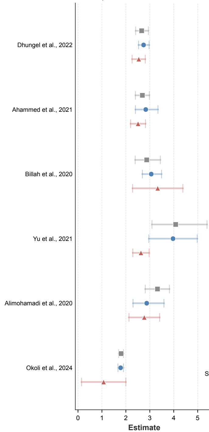
B Reproduction number
