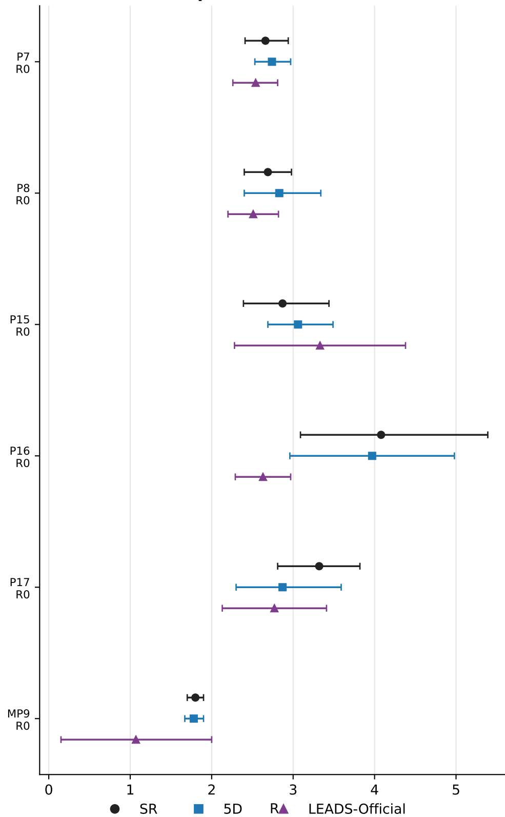
Reproduction number
