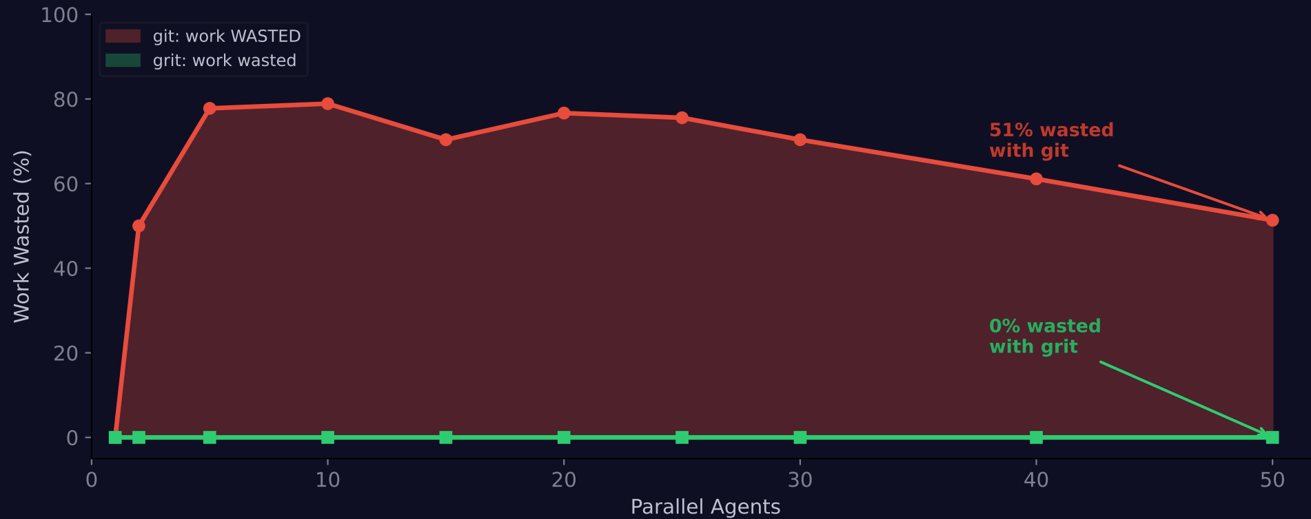
Developer/Agent Work Wasted to Conflicts
