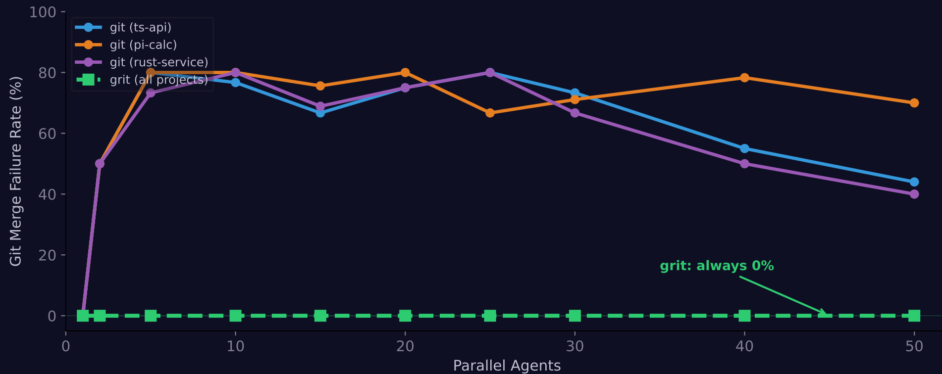
Merge Failure Rate: git vs grit
