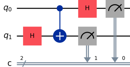
1.5a: circuit
