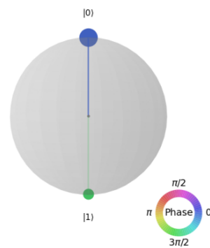
Q-sphere
