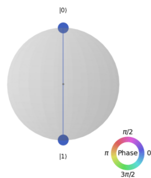
Q-sphere
