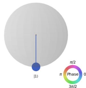
Q-sphere
