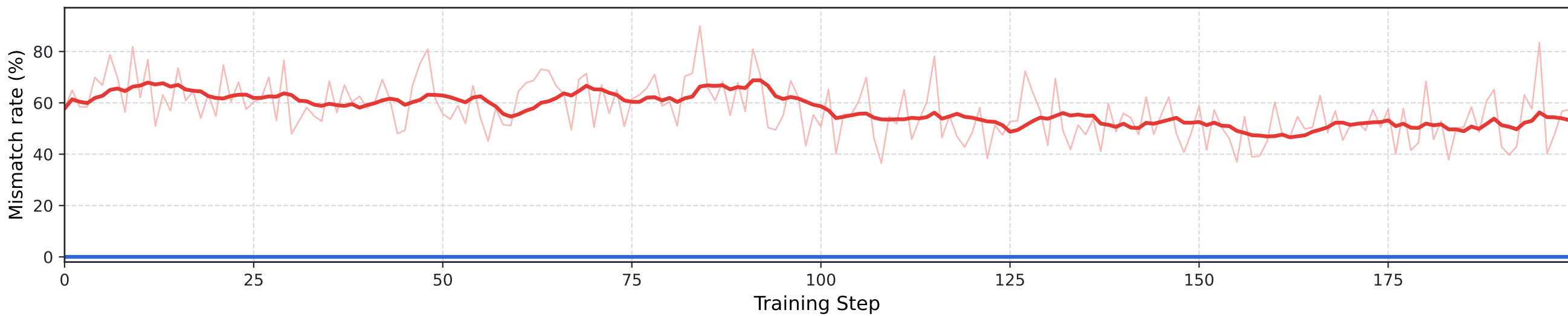
Bitwise log-probability mismatch rate
