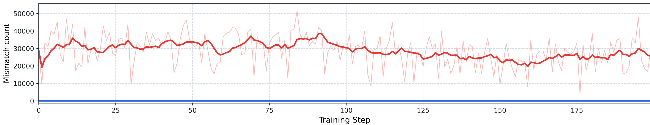
Bitwise log-probability mismatch count per step
