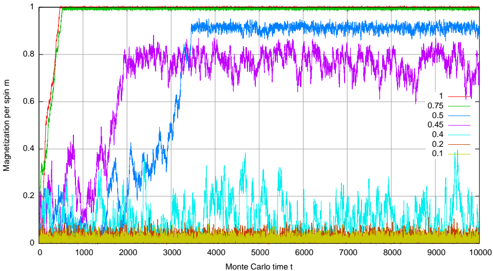
Magnetization versus MC time
