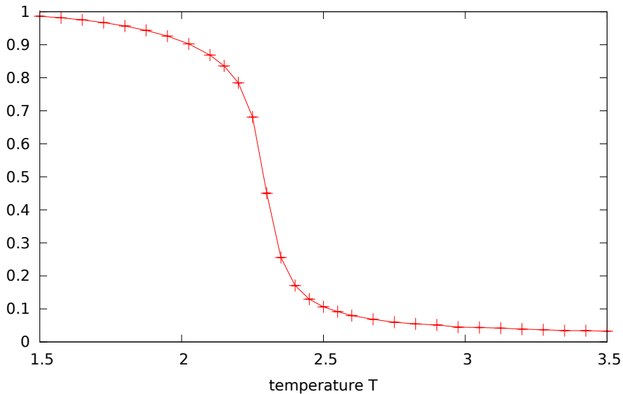
Average magnetization per spin
