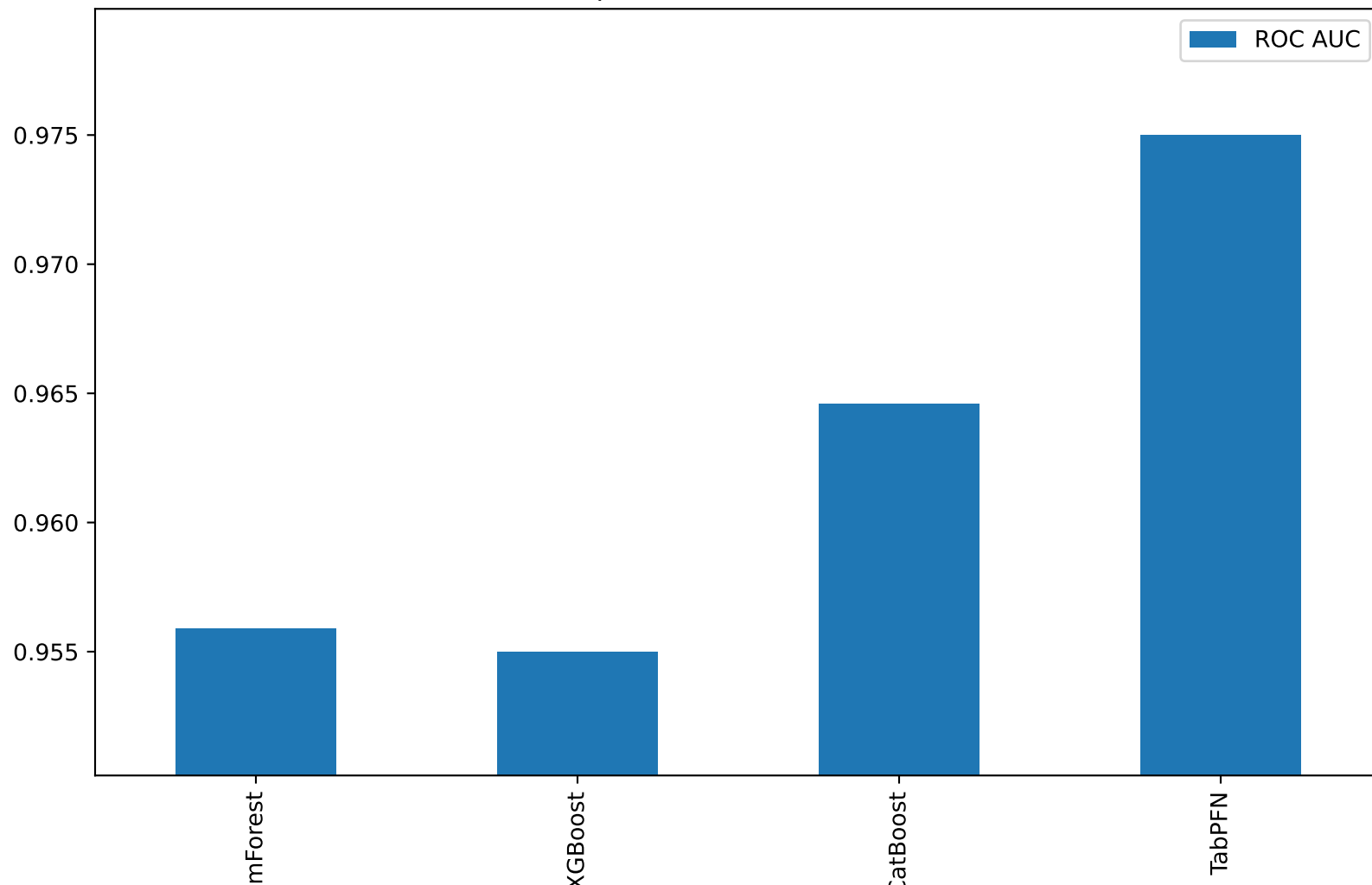
Model Comparison - 5-fold Cross-validation
