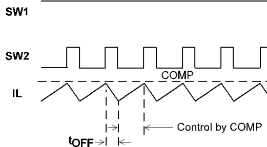
Figure 5: Boost Waveform
