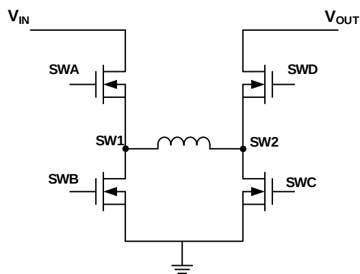
Figure 2: Buck-Boost Topology
