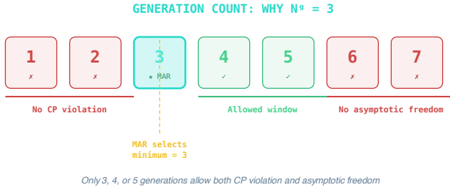
Figure 14.2: The generation-count window starts at three for intrinsic CP capability and closes above five from weak-sector ultraviolet consistency.
