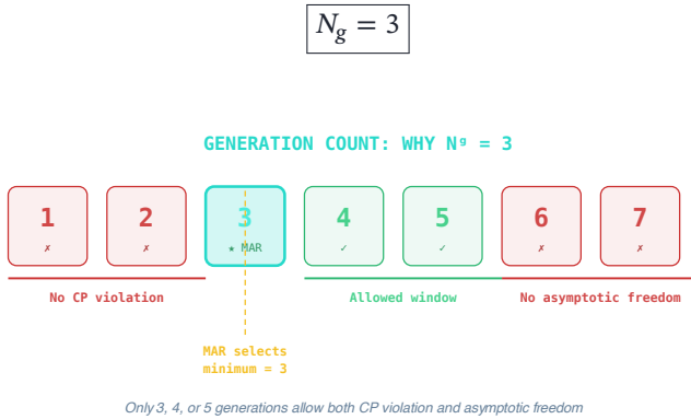
Figure 14.2: The generation-count window starts at three for intrinsic CP capability and closes above five from weak-sector ultraviolet consistency.
