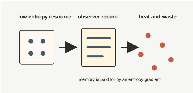
Figure 4.1: Record formation consumes low-entropy resources and exports the cost as heat and waste entropy.
