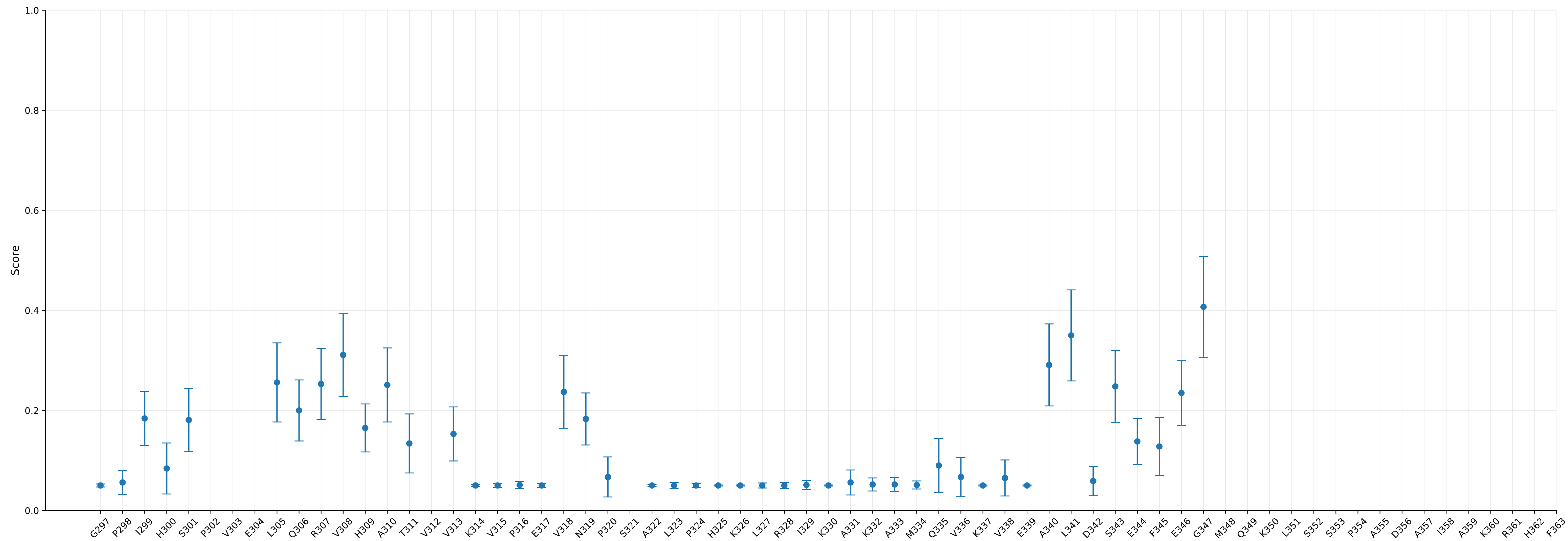
Postmean omega for residues between 297-363 in NFIL3 mouse
