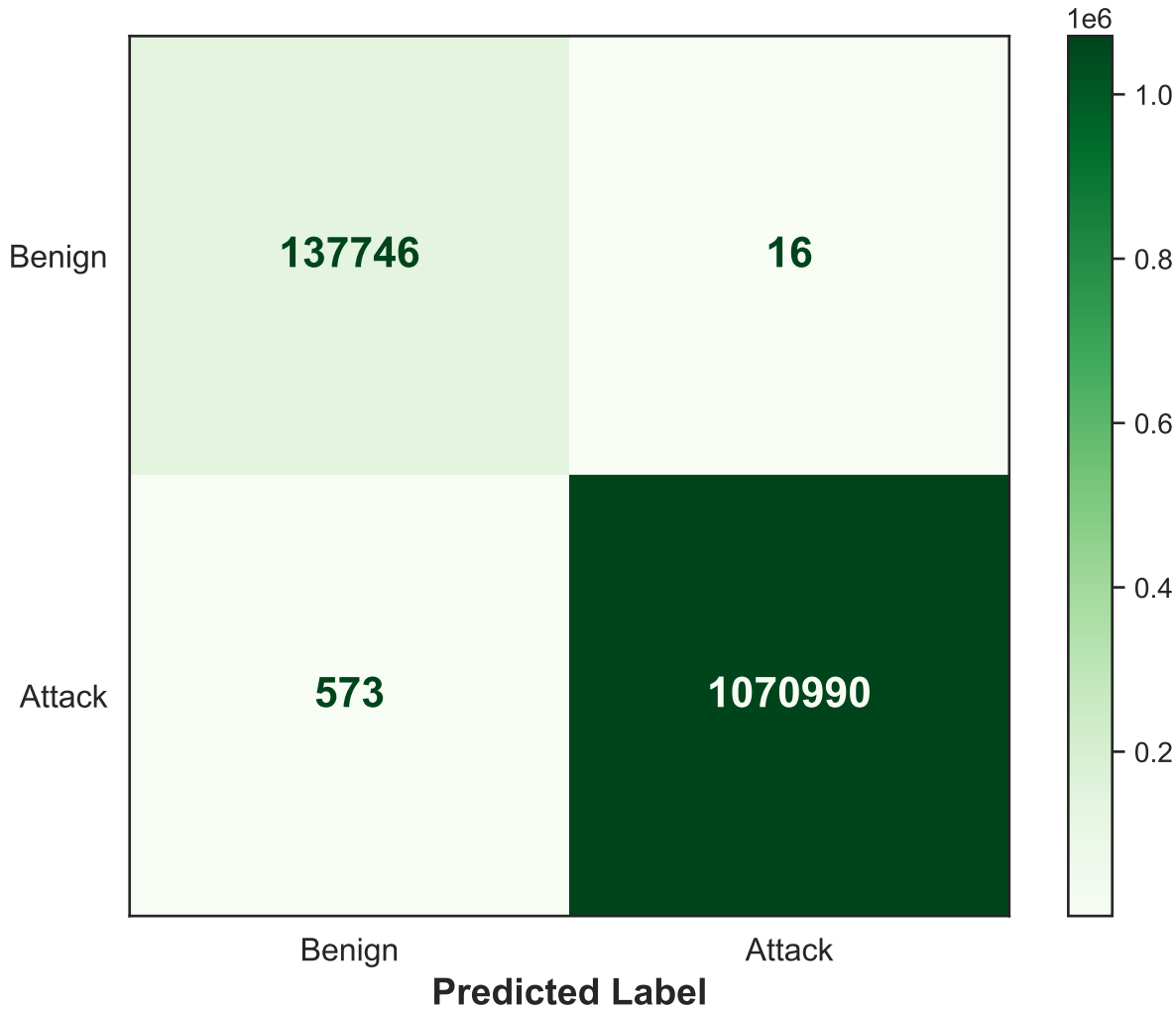
Confusion Matrix: Base Model Random Forest (Trees = 100, Depth = Unconstrained)
