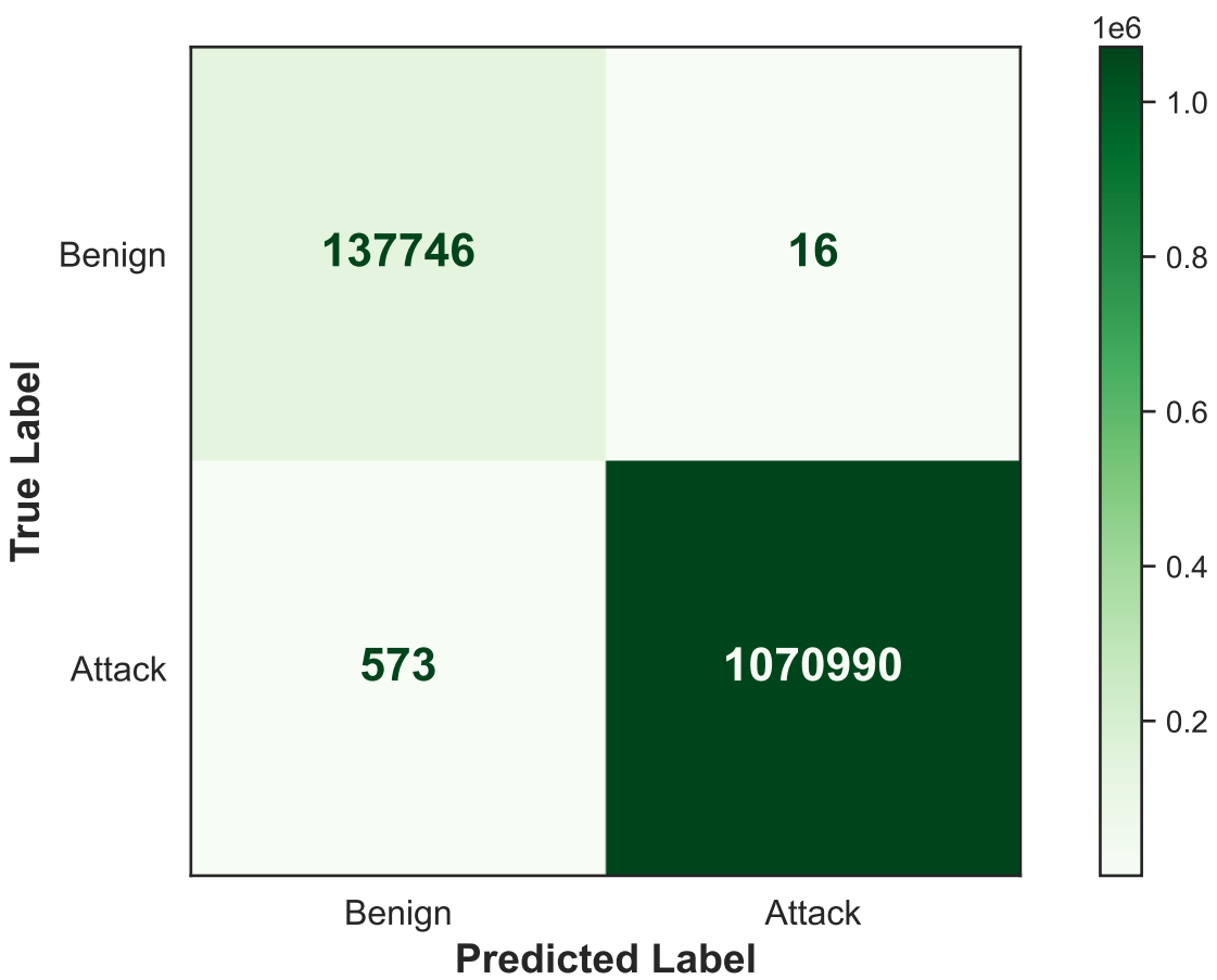
2. Meaningful Model (5 Features, 100 Trees)
