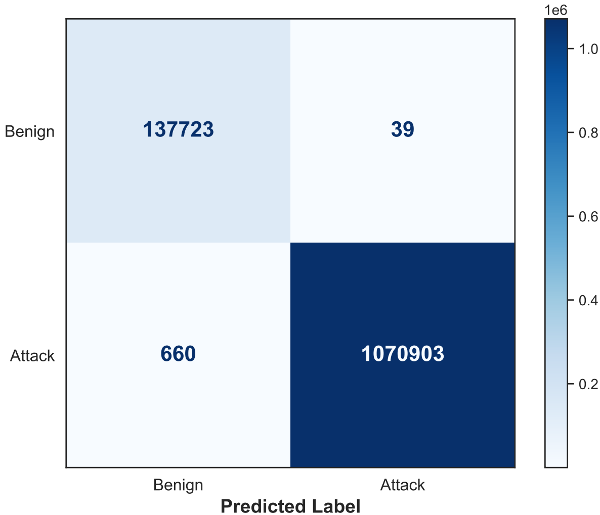
Confusion Matrix: 5-Feature Random Forest
