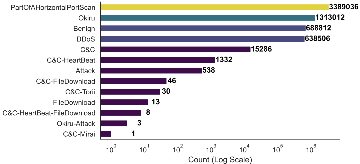
Distribution of Labels
