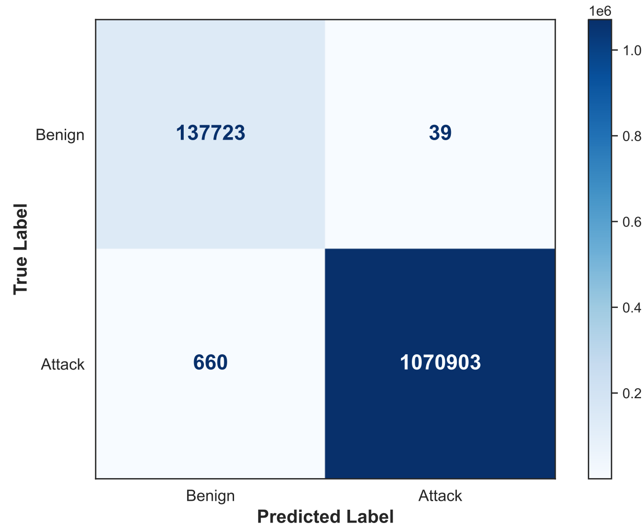
5-Feature Model
