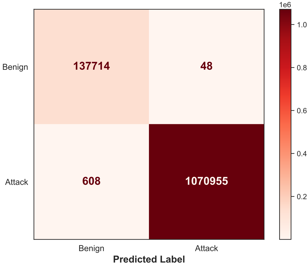
Confusion Matrix: Optimised Random Forest Model (Trees = 5, Depth = 15)
