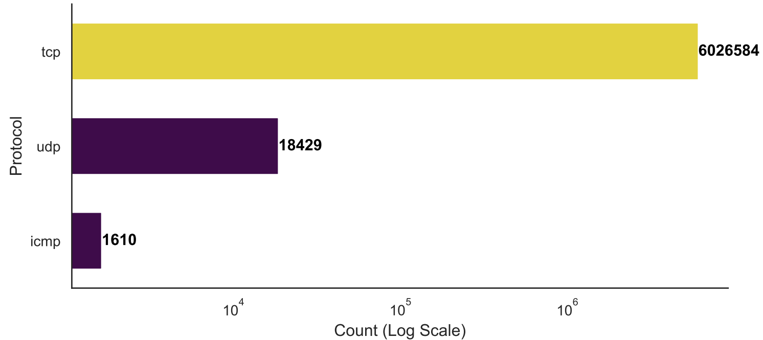
Distribution of Network Protocols
