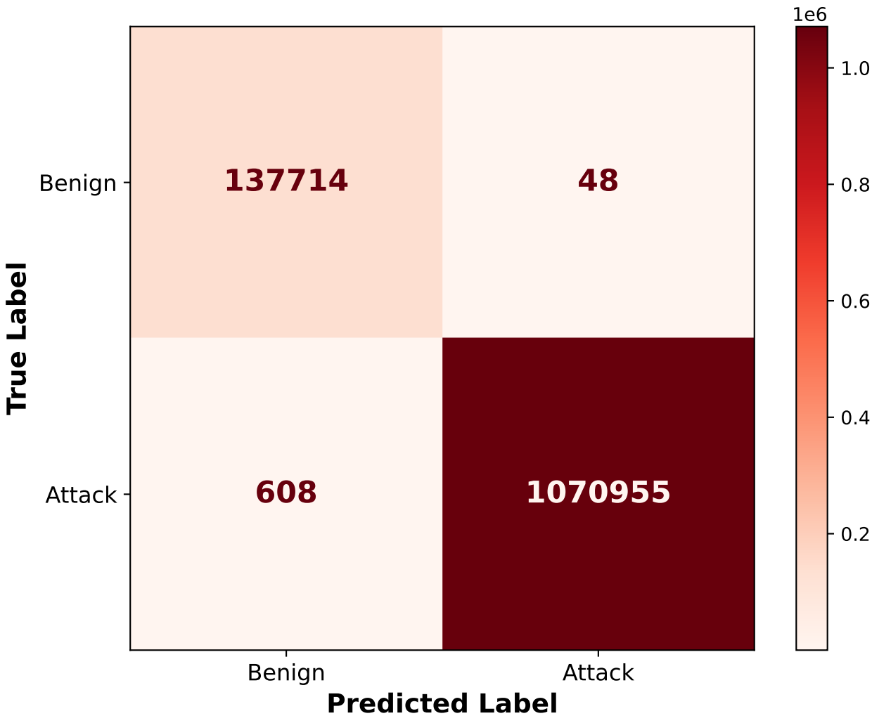
Confusion Matrix: Optimised RF Model (Trees = 5, Depth = 15)
