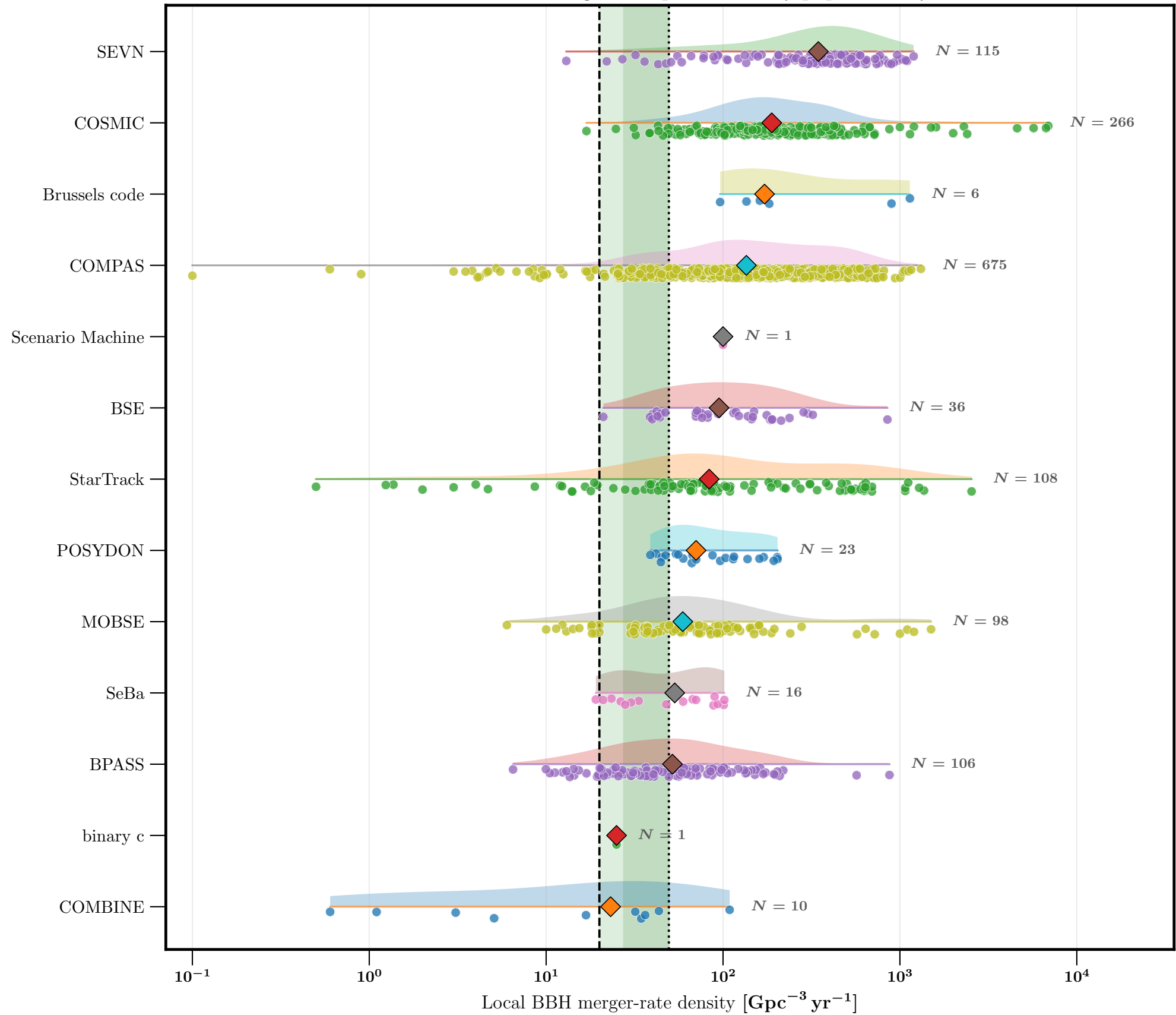
Distribution of local BBH merger-rate predictions by population-synthesis code
