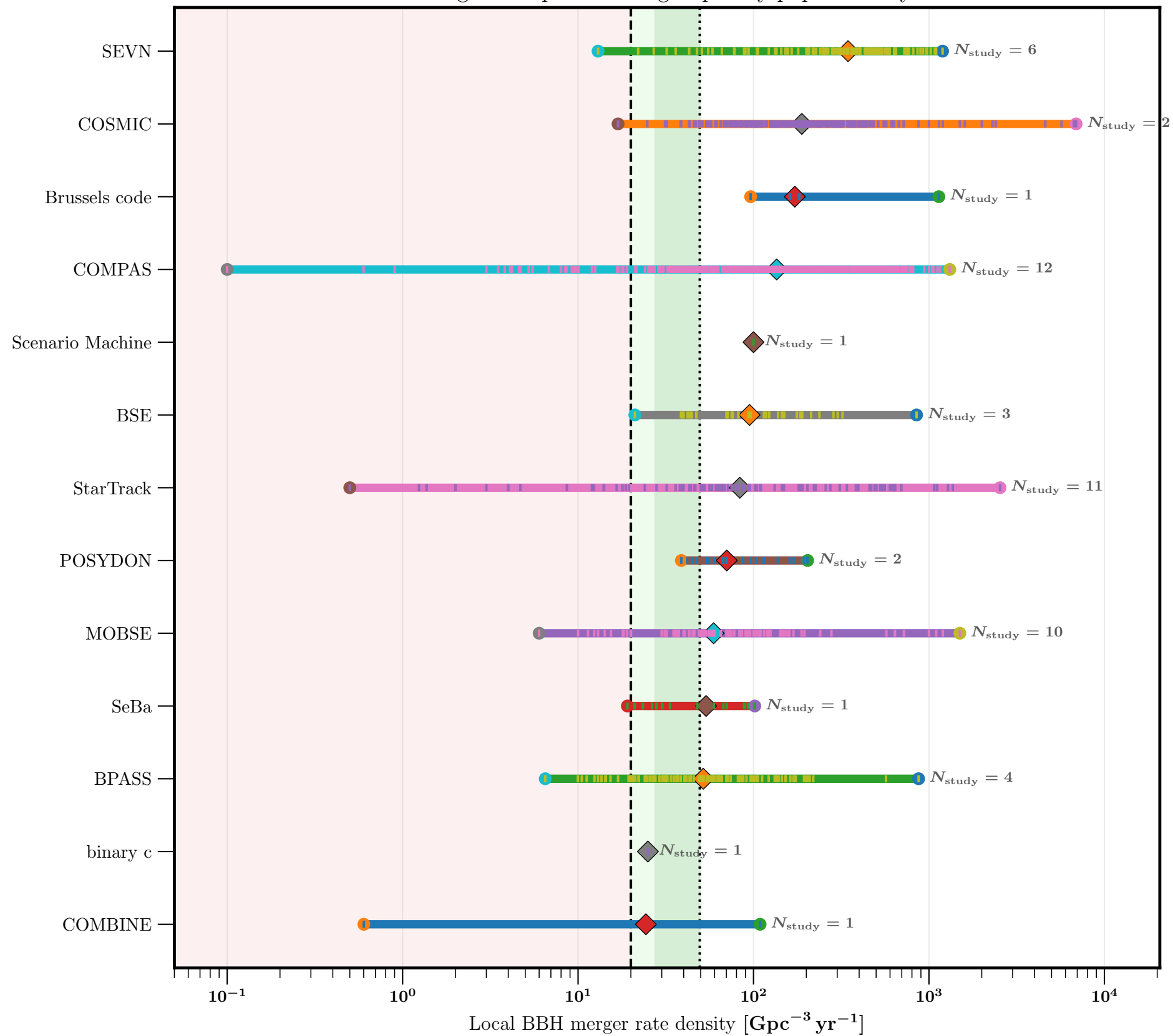
Local BBH merger-rate predictions grouped by population-synthesis code
