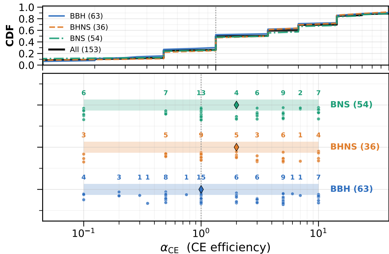
CE efficiency values by compact-object type
