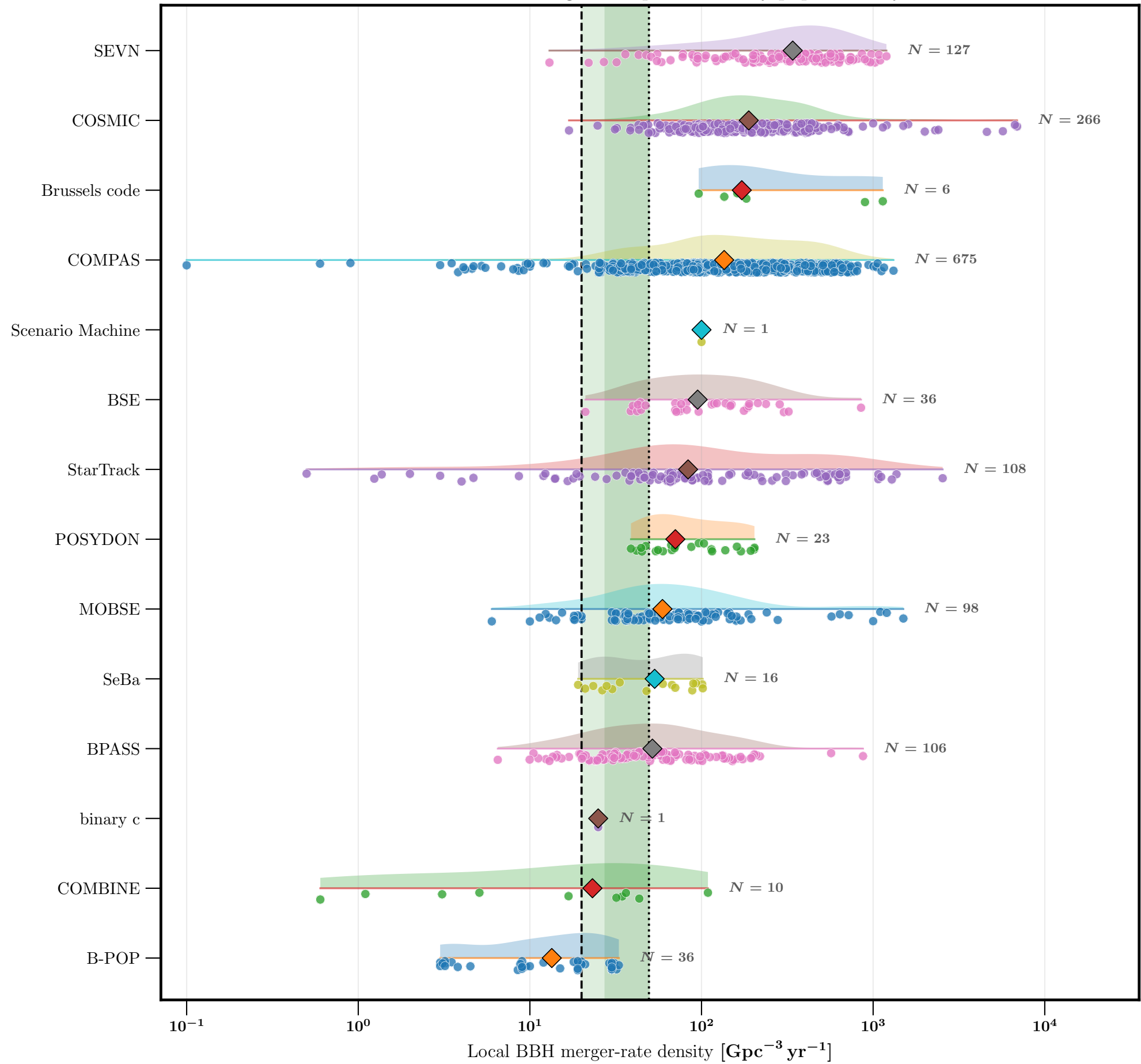
Distribution of local BBH merger-rate predictions by population-synthesis code
