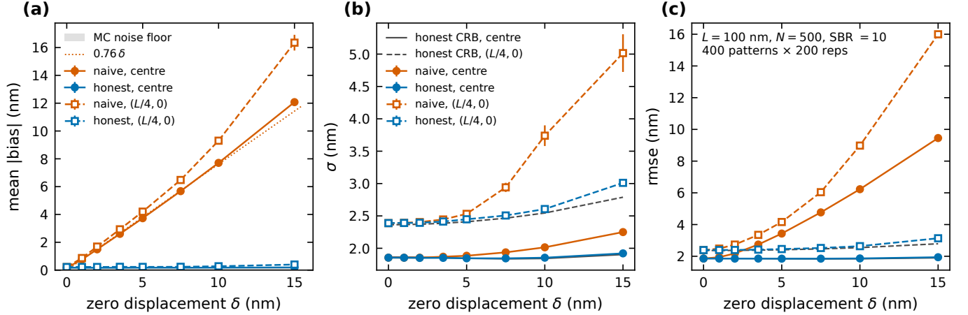
FIG. 8. TCP misalignment ( L = 100 nm, N = 500 , SBR = 10; all four zeros displaced by \delta in random directions; 400 patterns \times 200 repetitions; error bars are between-pattern SE). (a) Mean |\text{bias}| of the naive MLE (nominal pattern) and of the honest MLE (true pattern) versus \delta , at the centre and at (L/4, 0) , with the MC noise floor (grey band) and a straight line fitted to the naive centre points over all seven \delta values including \delta = 15 nm (dotted). The main slope estimate is the noise-free population value, 0.777 at the centre and 0.851 at (L/4, 0) , growing with \delta . (b) \sigma and (c) rmse versus \delta , with the CRB of the true pattern: at the centre the naive \sigma changes little and its loss is bias, whereas at (L/4, 0) the naive \sigma also grows, from 2.389 to 3.74 nm at \delta = 10 nm; the honest \sigma follows the CRB at the centre and lies slightly above it at (L/4, 0) .
