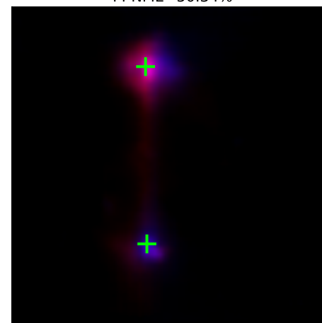
PI-NME=50.34%
