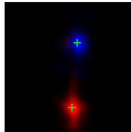
PI-NME=2.62%
