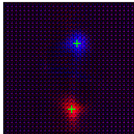
PI-NME=1.98%
