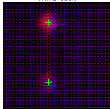
PI-NME=1.51%
