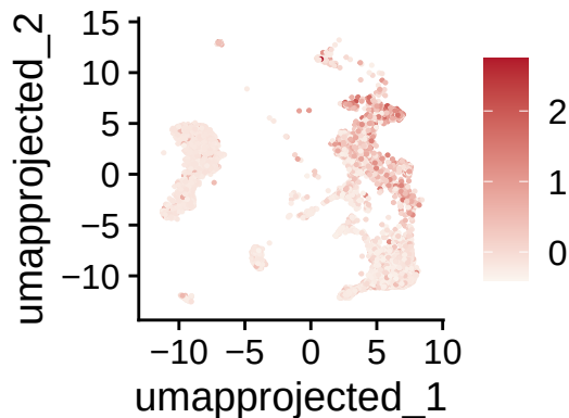
GATA2_MPP1_score1
