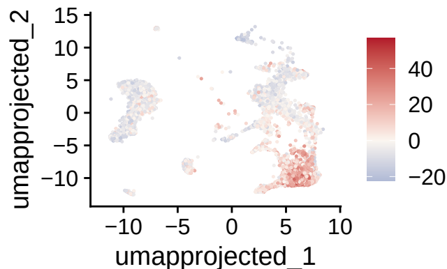
Factor_6_score
