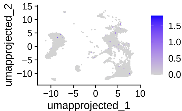
Factor_6_score
