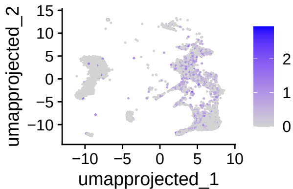
Factor_11_score
