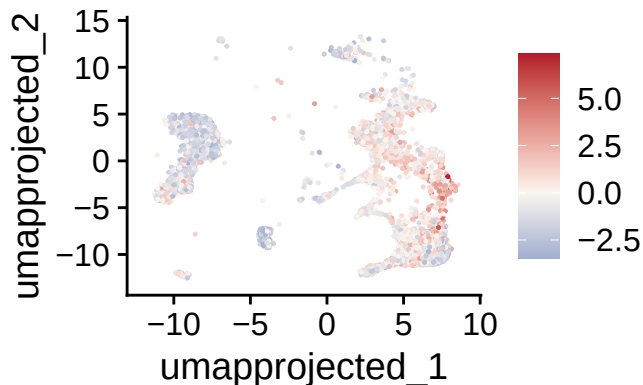
Factor_11_score
