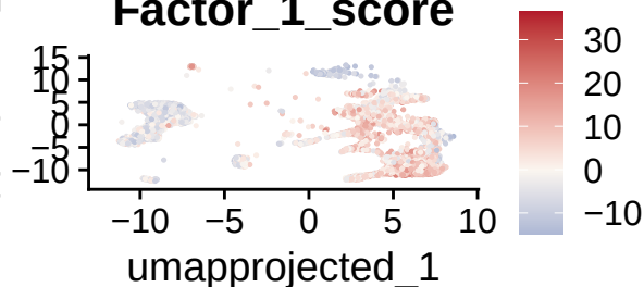
Factor_1_score
