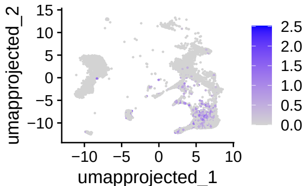
CD180
