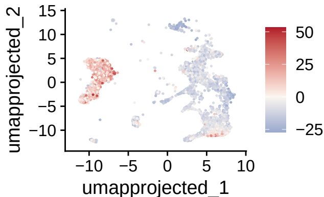
Factor_5_score
