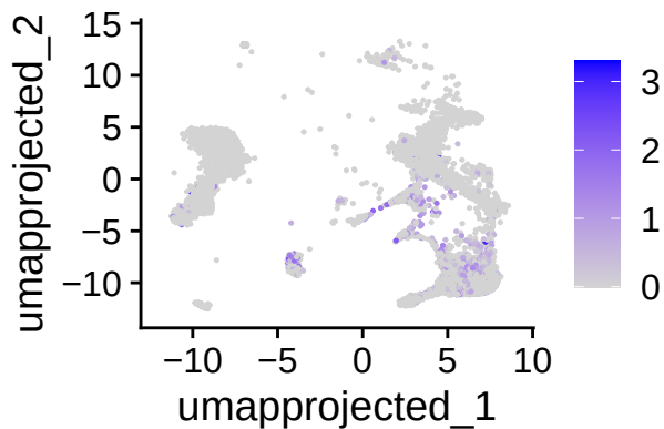
CD180
