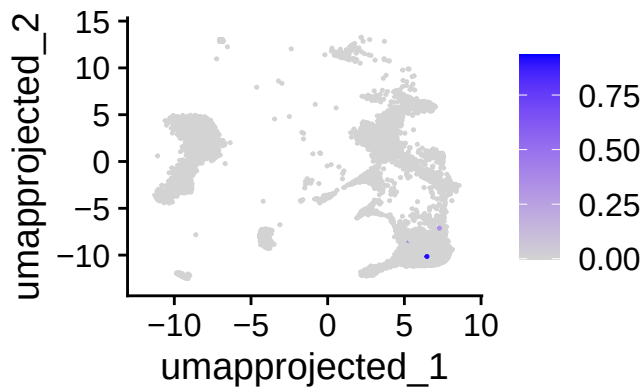
Factor_5_score
