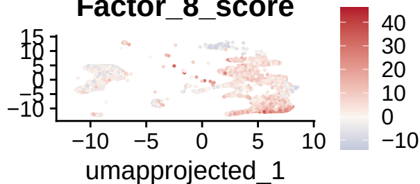
Factor_8_score
