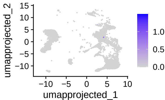
Factor_9_score
