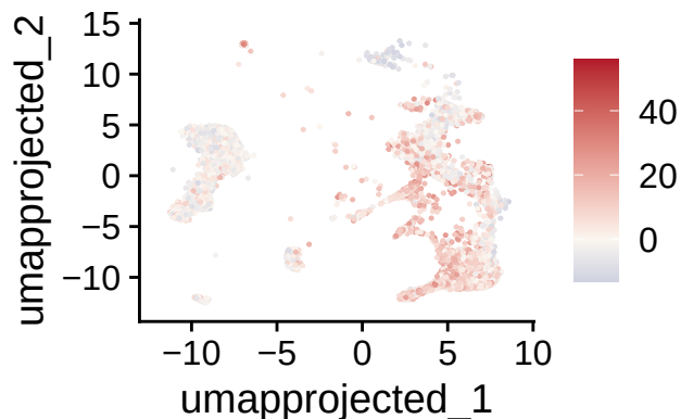
Factor_9_score
